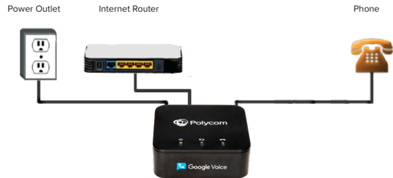
OBi200 Connections
