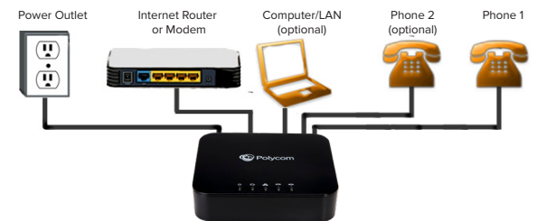
OBi302 Connections
